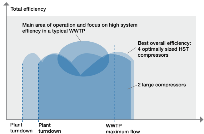
Four optimally sized HST compressors achieve better turndown.
